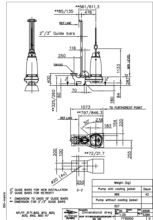
Figure 27: HT, P-installation
