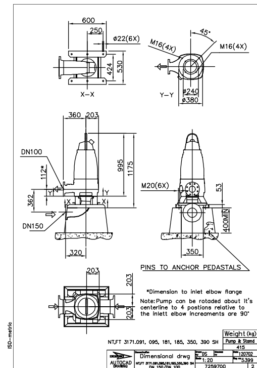
Figure 18: SH, T-installation
