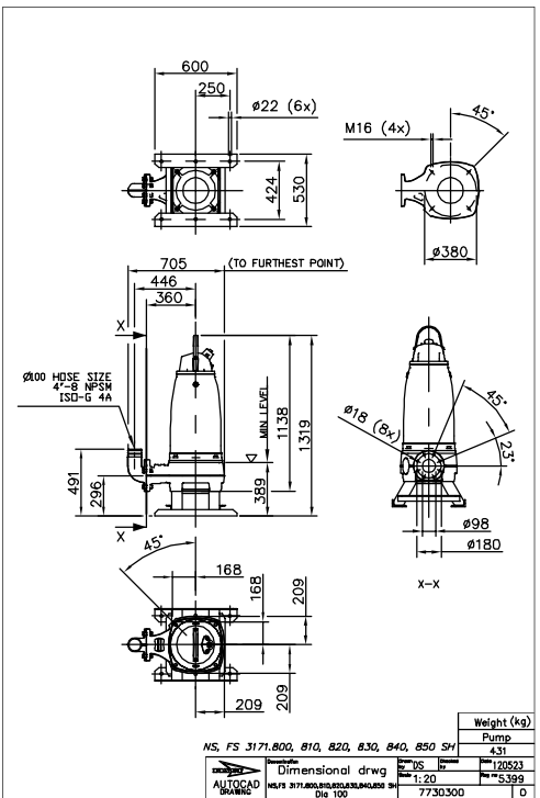
Figure 31: SH, S-installation
