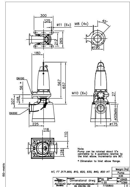
Figure 29: HT, T-installation
