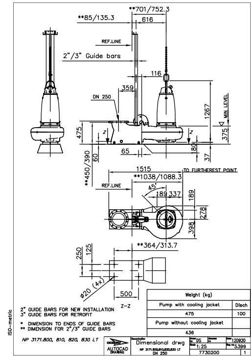
Figure 21: LT, P-installation
