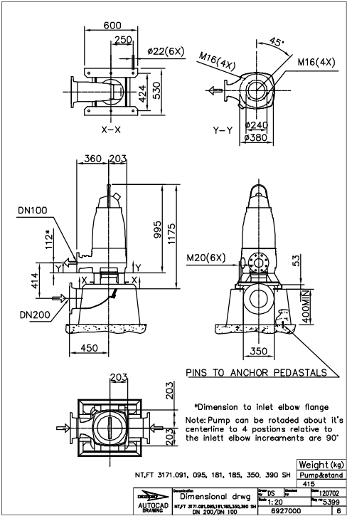
Figure 19: SH, T-installation
