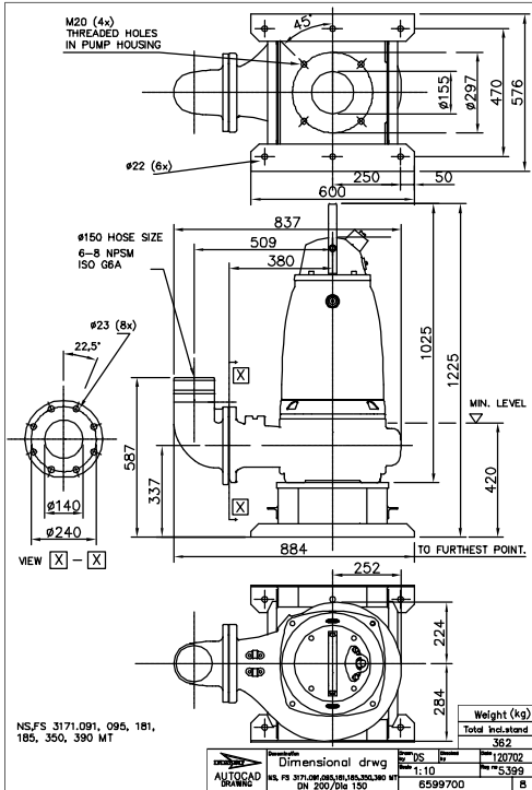
Figure 8: MT, S-installation
