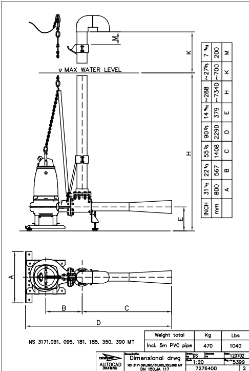
Figure 9: MT, S-installation
