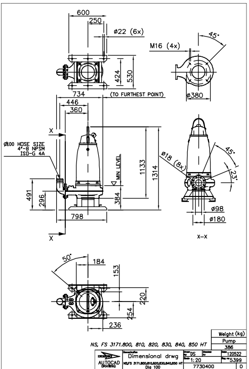
Figure 28: HT, S-installation
