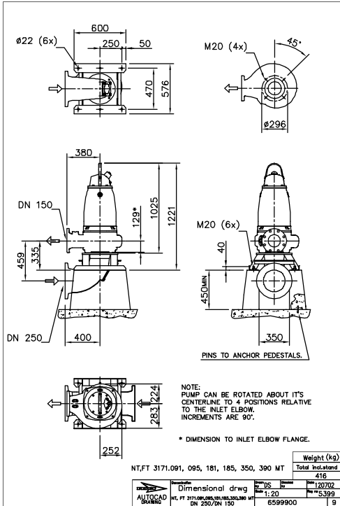
Figure 10: MT, T-installation
