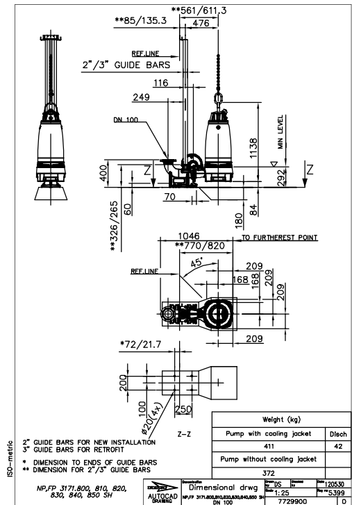
Figure 30: SH, P-installation
