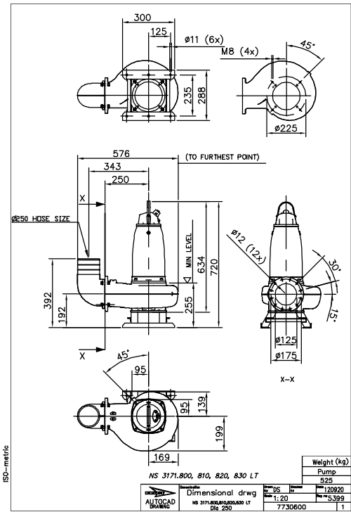
Figure 22: LT, S-installation
