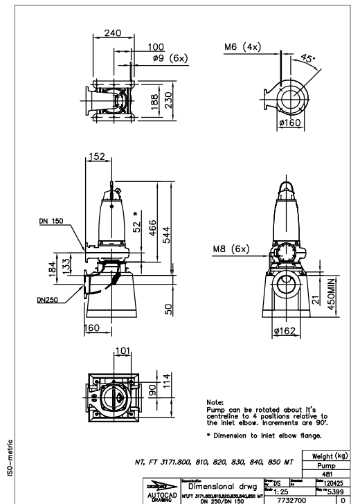
Figure 26: MT, T-installation
