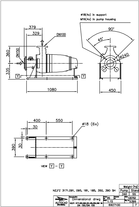
Figure 20: SH, Z-installation
